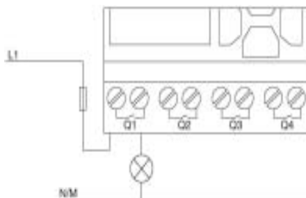
Fig 2.10 - Output relè
